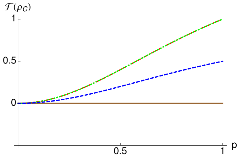
Figure 3. (Colors online) Quantum Fisher Information of the classically correlated state \rho_C with respect to four local Hamiltonians H^A = H_A \otimes \mathbb{I}_B, H^A = \sigma_x^A, y, z, (\sigma_x^A + \sigma_y^A)/\sqrt{2} . The parameter p determines the purity of the state. I depict the functions \mathcal{F}(\rho_C, \sigma_x^A) = 0 (brown, continuous line), \mathcal{F}(\rho_C, \sigma_y^A) = 2p^2/(1 + p^2) (red dot-dashed line), \mathcal{F}(\rho_C, \sigma_z^A) = 2p^2/(1 + p^2) (green dotted line), \mathcal{F}(\rho_C, (\sigma_x^A + \sigma_y^A)/\sqrt{2}) = p^2/(1 + p^2) (blue dashed line). Note that the state is unable to store information about the phase shift along the x -direction.
