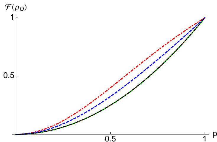
Figure 2. (Colors online) Quantum Fisher Information of the quantum correlated state \rho_Q with respect to four local Hamiltonians H^A = H_A \otimes \mathbb{I}_B , H^A = \sigma_x^A , y , z , (\sigma_x^A + \sigma_y^A)/\sqrt{2} . The parameter p determines the purity of the state. I depict the functions \mathcal{F}(\rho_Q, \sigma_x^A) = p^2 (brown, continuous line), \mathcal{F}(\rho_Q, \sigma_y^A) = 2p^2/(1+p^2) (red dot-dashed line), \mathcal{F}(\rho_Q, \sigma_z^A) = p^2 (green dotted line), \mathcal{F}(\rho_Q, (\sigma_x^A + \sigma_y^A)/\sqrt{2}) = p^2(p^2+3)/(2(p^2+1)) (blue dashed line), and the QIP given by the formula in [6] (black dot-dashed line). Note that the QFI is lower bounded by the discord of the state, which therefore ensures a minimum precision to the estimation.
