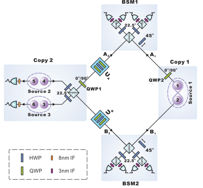
FIG. 2. Experimental setup. We prepare two copies of a Bell state |\phi^+\rangle by a laser-emitted ultraviolet pulse split into three beams pumping SPDC sources. The scheme guarantees that both copies are emitted by different sources. Conversely, in a two source setting, the fourfold coincidences in the BSMs could be generated by two photon pairs emitted from a single source, invalidating the experiment. The four terms of the mixture are obtained by rotating QWP1,2. Purity and overlap measurements are implemented via BSM schemes. A multichannel unit counts the sixfold coincidences (one detector fire in each output mode).
