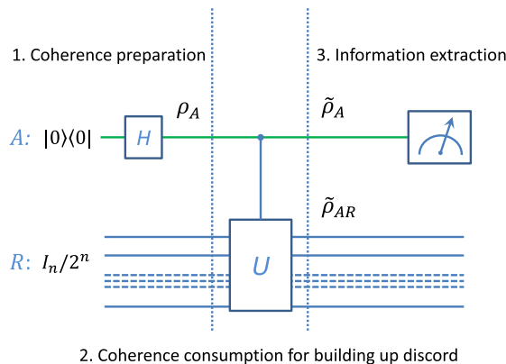
FIG. 3. DQC1 model. The algorithm consists of (1) preparing coherence in an ancillary pure qubit; (2) applying a controlled operation, which, in general, creates discord between the ancilla and a maximally mixed register by consuming the coherence of the ancilla; (3) obtaining information about \text{Tr}[U] by a polarization measurement in the ancilla: \langle \sigma_x + i\sigma_y \rangle_{\tilde{\rho}_A} = \text{Tr}[U]/2^n .
