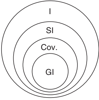
FIG. 4. Hierarchy of classes of incoherent operations: incoherent (I), strictly incoherent (SI), covariant (Cov.), and genuinely incoherent (GI).
