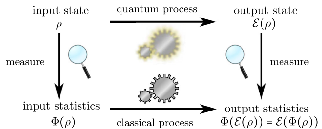
FIG. 1. Incoherent operations cannot create coherence; strictly incoherent operations, in addition, cannot use coherence. We depict here an SI operation \mathcal{E} , showing that all the initial coherence in the input \rho can be removed with a measurement \Phi (in the incoherent basis) without affecting the final measurement outcomes.
