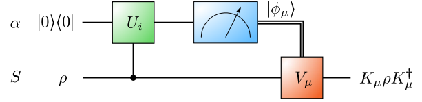
FIG. 3. Strictly incoherent operations on system S constructed by an incoherent unitary interaction with an ancilla \alpha . An operation is split into a controlled unitary \sum_i |i\rangle\langle i|_S \otimes (U_i)_\alpha followed by a measurement on the ancilla in a basis |\phi_\mu\rangle and an incoherent unitary V_\mu on the system conditioned on the measurement outcome \mu .
