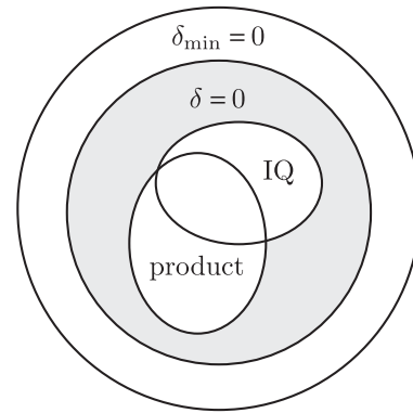
FIG. 5. Schematic illustration of the sets for which the following quantities vanish: \delta_{\min}(B|A) (CQ states), \delta(B|A) (Result 2), C(B|A) (IQ states), and I(A:B) (product states). When A is a qubit, the shaded region is empty.
