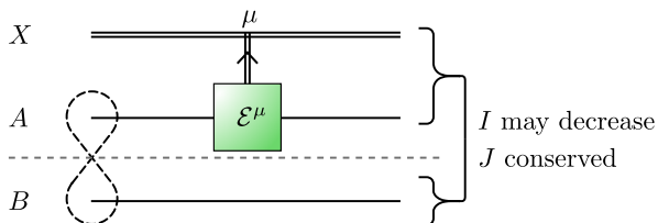
FIG. 6. Circuit representation of a local SI operation on a bipartite system AB . When an outcome \mathcal{E}^{\mu} is obtained by selecting a result \mu from the ancilla measurement in the dilation (Result 1), \mu is recorded in a classical memory X . Retaining X , the total correlations I(AX:B) cannot increase, but the classical correlations J(B|AX) are conserved.
