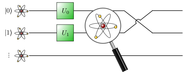
FIG. 2. Strictly incoherent operations viewed as operations on a particle traveling through an interferometer. The different branches |i\rangle span the Hilbert space \mathcal{H}_B , while the internal state of the particle has Hilbert space \mathcal{H}_I . The operations are built up by combining path-dependent unitary operations U_i on and measurements of the internal state of the particle, as well as permutations of the paths.
