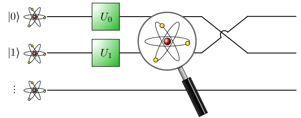
FIG. 2. Strictly incoherent operations viewed as operations on a particle traveling through an interferometer. The different branches |i\rangle span the Hilbert space \mathcal{H}_B , while the internal state of the particle has Hilbert space \mathcal{H}_I . The operations are built up by combining path-dependent unitary operations U_i on and measurements of the internal state of the particle, as well as permutations of the paths.
