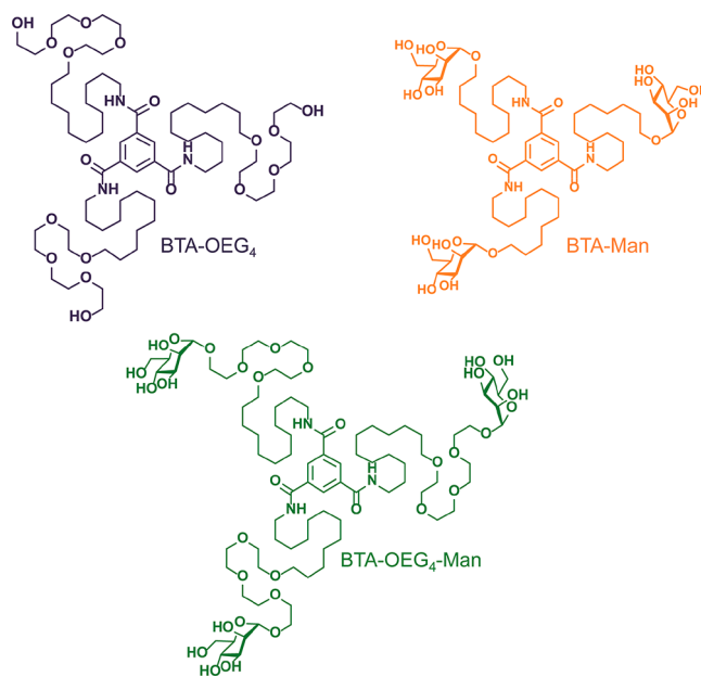
Scheme 1. Chemical Structure of the Water-Compatible BTA Monomers Selected for This Study
