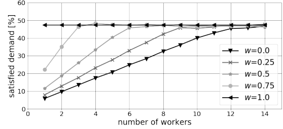
Fig. 8: Minneapolis - percentage of satisfied demand, varying number of workers and users willingness ( t_{\text{reach}} = 30 minutes)
