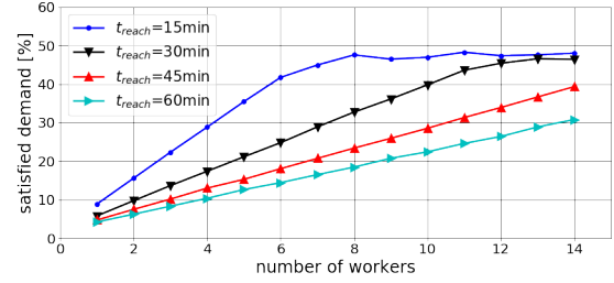
Fig. 7: Minneapolis - percentage of satisfied demand, varying number of workers and average reach time
