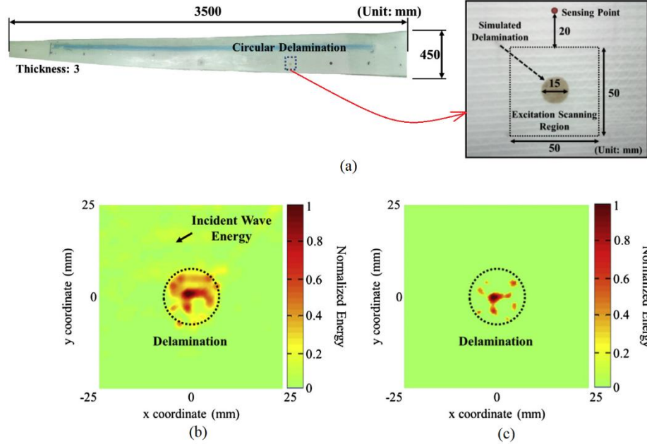
Fig. 12. (a) composite blade of wind turbine, (b) CTWE image, and (c) CSWE image [67]
