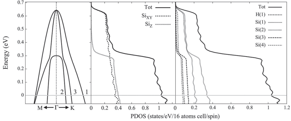
Fig. 6. – Electronic structure analysis of the hydrogenated silicon (111) surface at n_{dop} = 6 \cdot 10^{14} \text{ cm}^{-2} . First panel: electronic dispersion along high-symmetry directions of the First Brillouin Zone ( \mathbf{M}-\Gamma-\mathbf{K} ). Second panel: partial density of states (PDOS) depicting the planar ( XY ) and out-of-plane ( Z ) character of the electronic bands. Third panel: partial density of states (PDOS) showing the contribution of the atomic layers involved in the field-effect doping (as labelled in fig. 1). The horizontal grey line is the Fermi level, here set to E_F = 0 . DOS and PDOS are in units of states/eV/16 atoms cell/spin.
