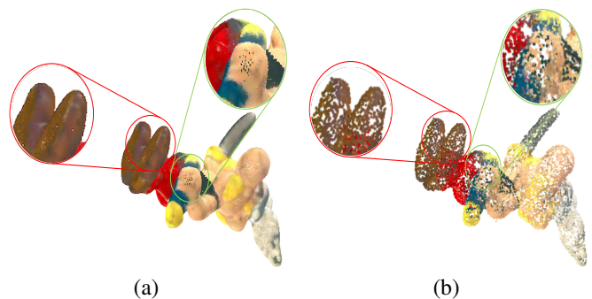
Fig. 1: Asterix model: (a) Ground-truth, (b) denoised with IBR [6]. The noisy points are moved towards their nearest neighbors rather than their original positions, generating holes in the denoised point cloud.
