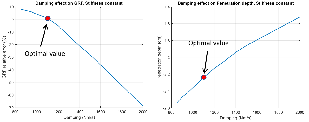
Figure 8 Sensitivity analysis: damping effects on GRF and penetration depth
