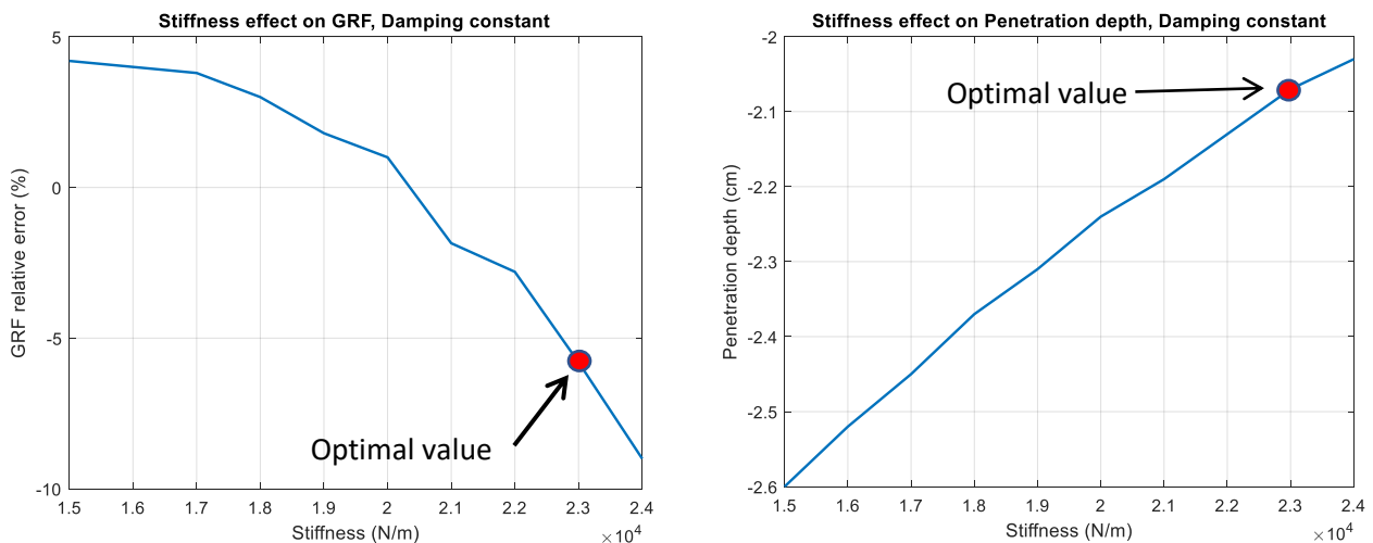
Figure 7 Sensitivity analysis: stiffness effects on GRF and penetration depth
