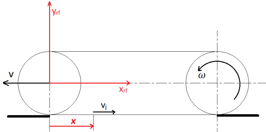
Figure 11. Coordinate system for traction force equation integration.
