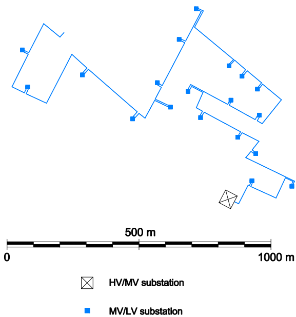
Figure 8. Feeder 3.
