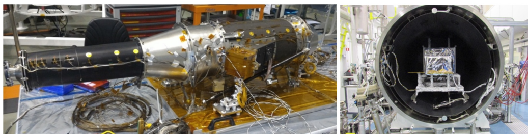
Fig. 25. Metis structural thermal model prepared for the vacuum thermal-balance test with temperature sensors installed inside and on the external surface ( left ). Metis structural thermal model inside the thermal-vacuum chamber endowed with Sun simulator, at ESTEC/ESA ( right ).
