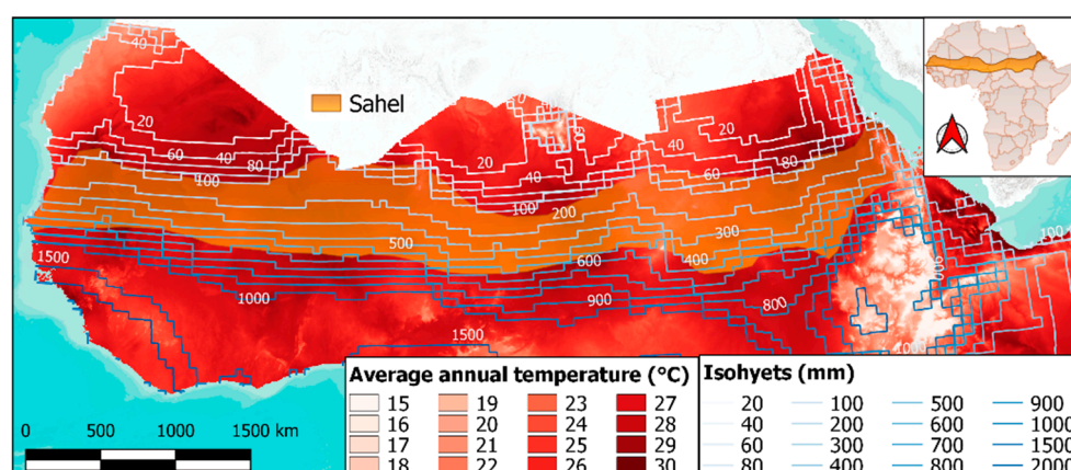
Figure 1. Geolocation of the Sahelian strip. Long-term climate data: average temperature (1970–2000) and isohyets (1960–2014) of the sub-Saharan area [37,42].
