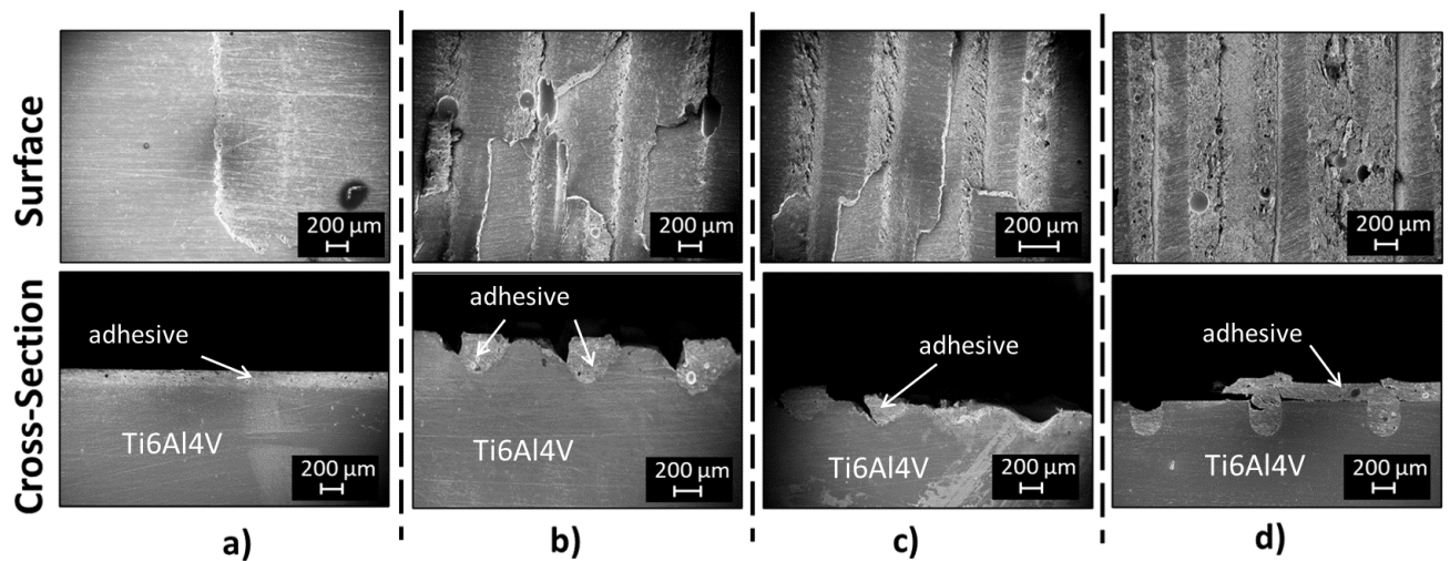
Figure 8 Joint fracture analysis at higher magnification: top view and cross – sectional micrographs (a) Unmodified surface, (b) Semi-overlapped V-shaped micro-slot surface, (c) Interlocked semi-circle shaped micro-slot surface, (d) Semi-overlapped U-shaped micro-slot surface; all the tested samples were oriented perpendicular to the load.
