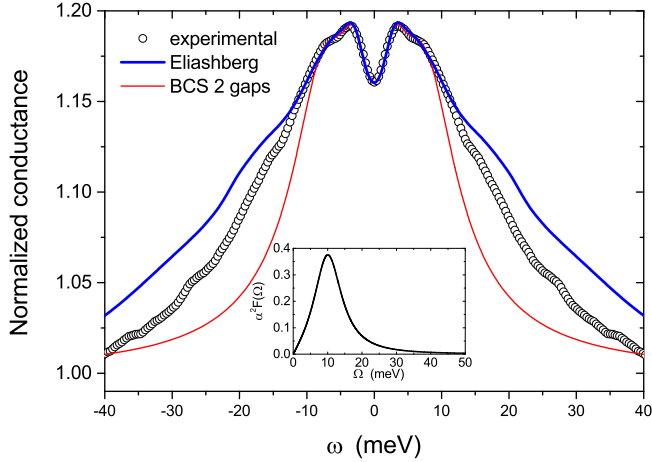
FIG. 9. Open circles: experimental data reported in Fig. 4(b). Blue line: calculated curve after inserting into the three-band BTK-like model the energy-dependent order parameters, calculated by solving the Eliashberg equations. The red line is a fit of the theoretical curve with a two-band BCS-based BTK model (with constant gaps), which reproduces the same gap values as in Fig. 4(b) (red curve). The inset shows the electron-boson spectral function for the antiferromagnetic spin fluctuations, here normalized to have \lambda = 1 .
