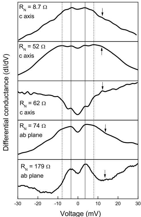
FIG. 2. Low-temperature (2.7 K) conductance curves for various contacts made on the same single crystal. Despite the different shapes, all the curves display structures (maxima, shoulders, slope changes) at approximately the same positions, as indicated by the vertical lines at \pm 3.5 mV and \pm 7.5 mV. Arrows indicate structures related to the strong electron-boson coupling.
