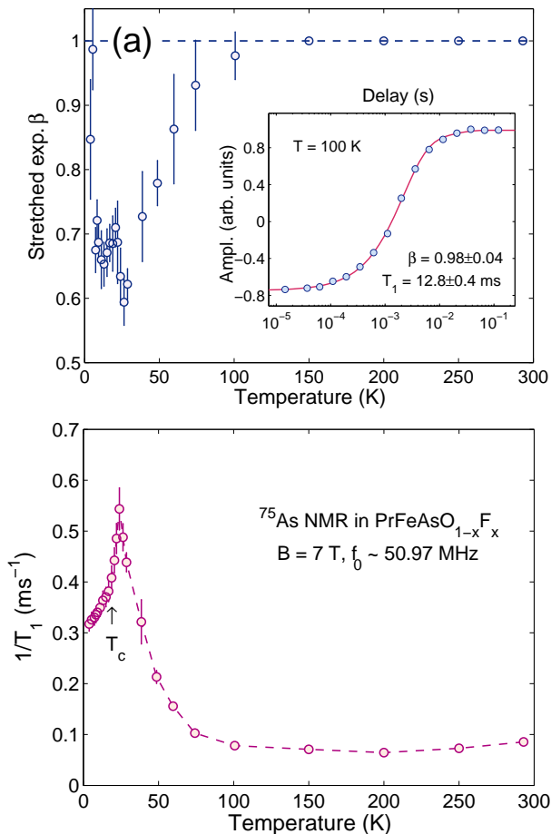
FIG. 8. (a) Stretched-exponential coefficient \beta vs. temperature. Below 100 K, \beta deviates increasingly from 1 (dashed line). Inset: recovery of magnetization during a typical ^{75}\text{As} NMR T_1 measurement at 100 K. (b) Temperature dependence of the ^{75}\text{As} NMR relaxation rate 1/T_1 , measured at 7 T. Below 100 K, the relaxation (dominated by spin fluctuations) becomes increasingly faster and peaks at 24 K, i.e., well above T_c (see arrow). In the superconducting phase, the behavior is not exponential and 1/T_1 saturates at a nonzero value, here reflecting the presence of \text{Pr}^{3+} magnetic ions.
