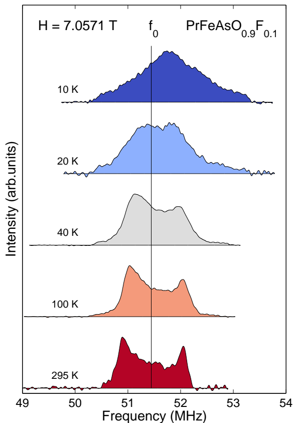
FIG. 7. Frequency-swept ^{75}\text{As} NMR spectra in \text{PrFeAs}(\text{O},\text{F}) , measured at 7 T. The lines refer to the ^{75}\text{As} central transition, whose features reflect a second-order quadrupole broadening. While down to T_c the line width is relatively insensitive to temperature, its position shifts towards higher frequencies (especially below T_c ). The vertical line indicates the reference ^{75}\text{As} -NMR frequency.
