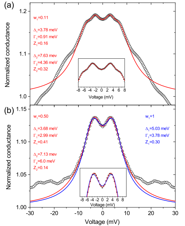
FIG. 5. (a) Normalized differential conductance at 2.7 K (circles) and relevant fit (red line) for a c -axis contact with a resistance of 8.7 Ω. (b) Open circles: low-temperature (2.7 K) conductance spectrum of a 179-Ω, ab -plane contact, divided by the normal-state conductance curve without any shift. The blue line is a single-gap fit, while the red curve is a two-gap fit, both made with |V_{\text{max}}| = 10 mV. The inset shows a closeup of the low-bias region.
