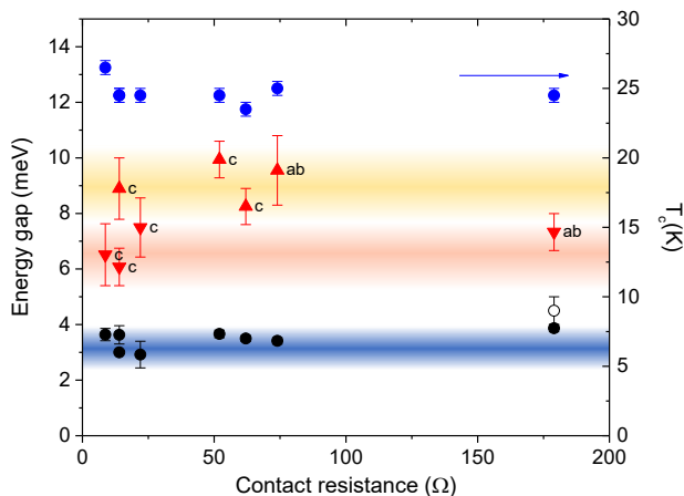
FIG. 6. Energy gaps (red and black solid symbols) and Andreev critical temperature (blue symbols) as a function of the contact resistance. The open symbol represents the result of a single-gap fit of the curve shown in Fig. 5(b). The labels indicate the type of contact (i.e., with current parallel to the c axis or to the ab planes).
