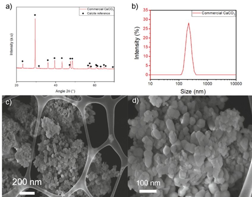
Fig. 2. \text{CaCO}_3 particles characterization. (a) X-Ray Diffraction; (b) Particle size Distribution; (c) (d) FESEM micrographs.
