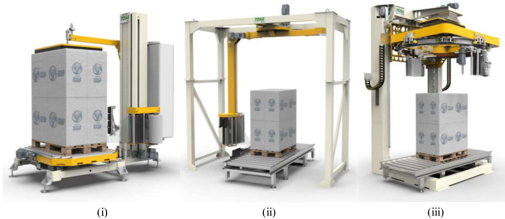
Figure 1 – Illustration of the three main categories of wrapping machines: (i) turn table, (ii) rotating arm and (iii) rotating ring.
