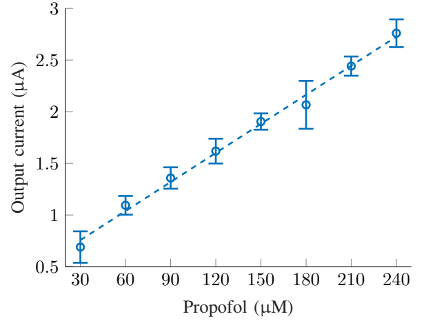
Fig. 5: Inter-electrodes calibration curve of proposed needle-shaped sensor measuring propofol in human serum.
