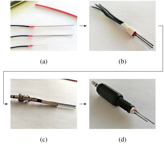
Fig. 3: Sensor assembly process: pencil leads and Pt wire connected to soldering wire through heat-shrink tubes (a), joint together (b), soldered to audio jack connector (c), closed and cut to length to form the complete sensor with integrated audio jack connector for point-of-care applications (d).
