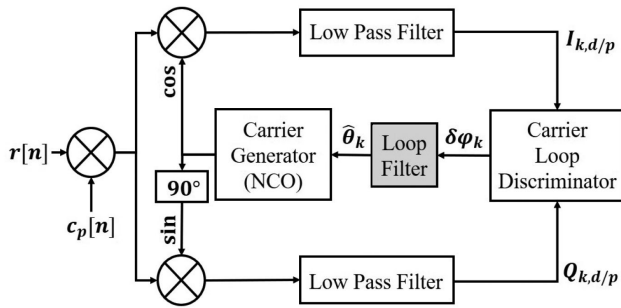
Fig. 9. Signal carrier tracking block diagram.
