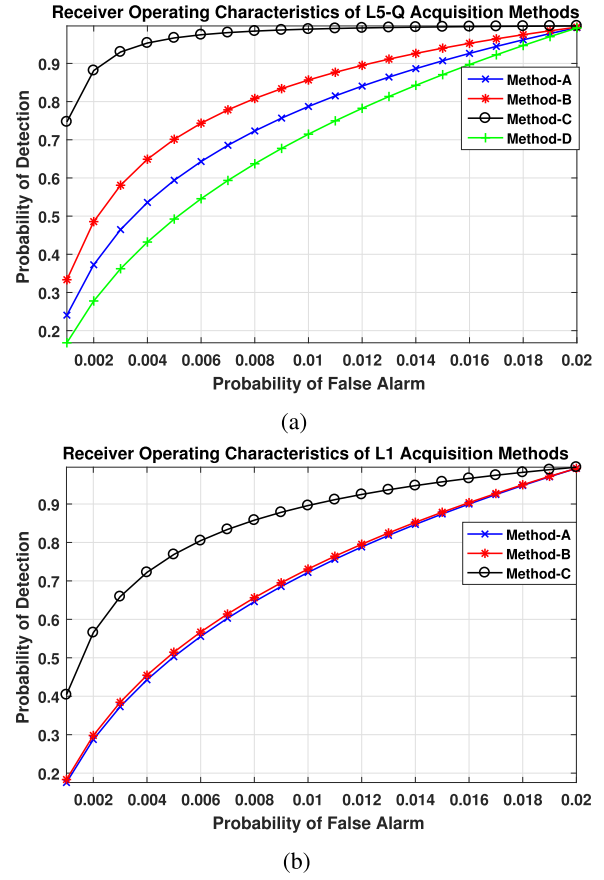
Fig. 5. ROC curves of the implemented methods for GPS L1 C/A, L5 signals under no-scintillation. (a) GPS L5 pilot signal ( C/N_0 = 51 dBHz). (b) GPS L1 C/A signal ( C/N_0 = 48 dBHz).
