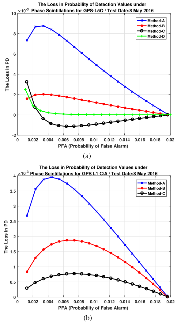
Fig. 6. Loss in PD of the acquisition methods for GPS L1 C/A, L5 signals under phase scintillation—May 8, 2016. (a) GPS L5 pilot signal. (b) GPS L1 C/A signal.
