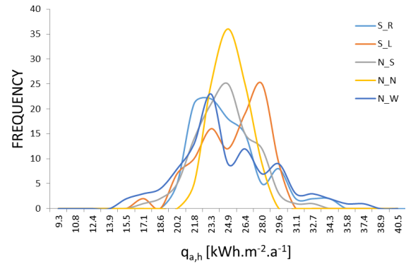
Fig. 5 – Computed annual heating demand distributions as a consequence of assumed input variable distributions (see Fig. 4)
