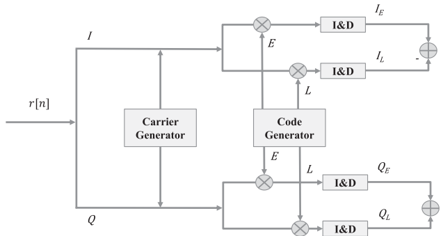
Fig. 3. Open-loop code discriminator.
