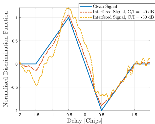
Fig. 13. S-Curve for BPSK (GPS L1, PRN 1) distorted by a linear chirp, with B_n = 16 \text{ MHz} , T_p = 20 \mu\text{s} , and f_c = 1 \text{ MHz} .
