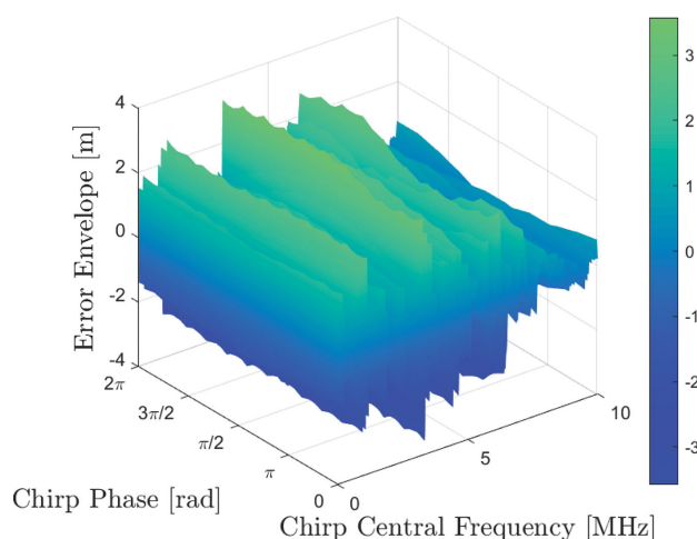
Fig. 14. Error envelope for BPSK (GPS L1, PRN 1) versus chirp phase and chirp central frequency, with B_n = 16 \text{ MHz} , T_p = 20 \mu\text{s} , and C/I = 0 \text{ dB} .
