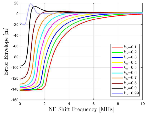
Fig. 11. NEE for BOC (1, 1), with \Delta = 1 chip.
