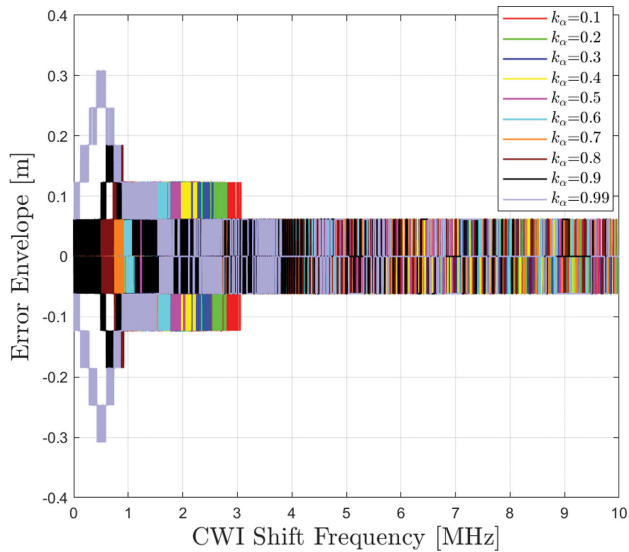
Fig. 9. IEE for CWI after NF mitigation and compensation process for BPSK (GPS L1, PRN 1).
