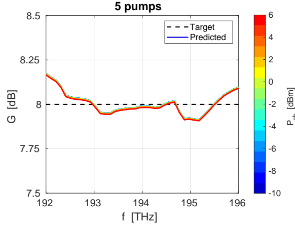
Fig. 16. Gain profile for increasing per-channel input signal power levels from -10 dBm to 6 dBm.
