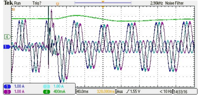
Fig. 20. Oscilloscope screenshot of phase currents (phases a1, a2, a3 ; 1 A on oscilloscope = 0.25 A of real current) and electromagnetic torque measured with torque meter (400 mA = 0.5 Nm of real torque). Waveforms filtered with a 2.9 kHz filter.
