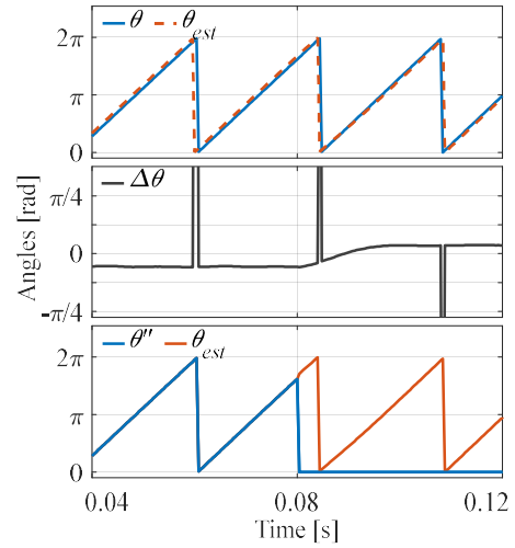
Fig. 21. Position angle analysis: actual and estimated angles and position estimation error (zoomed extracts around the instant of fault; \theta' stands for encoder position signal \theta as seen by the control system).
