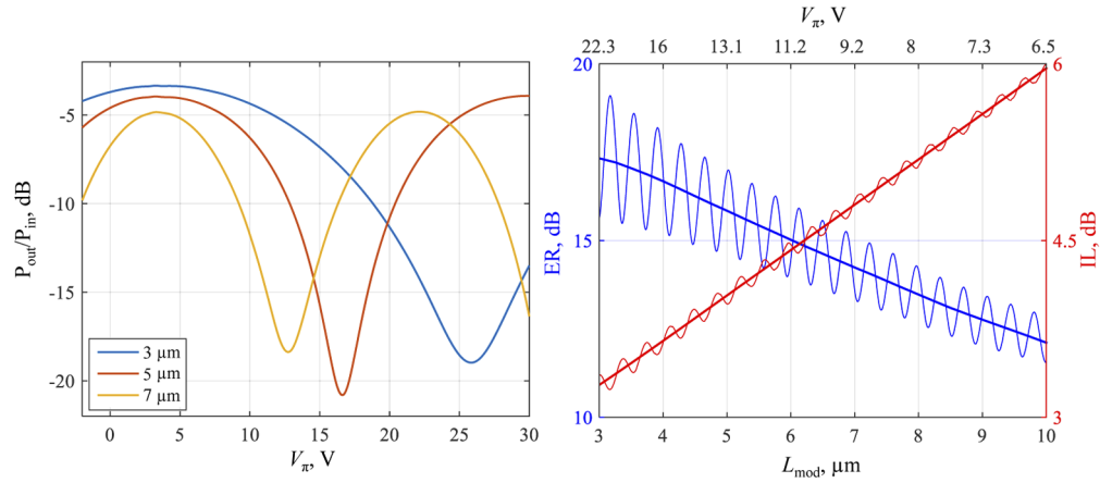
Fig. 11. Left: plot of the MZM response for different modulator lengths: the blue, red, and orange curves refer to L_{mod} = 3 \mu m , 5 \mu m , and 7 \mu m , respectively. Right: plot of the extinction ratio (ER, thinner blue curve, referred to the left axis) and insertion loss (IL, thinner red curve, referred to the right axis) as a function of L_{mod} , obtained from S_{21} from the simulated modulator response Eq. (10). The thicker curves are used to emphasize the average trends. The top abscissas axis shows the corresponding V_{\pi} .
