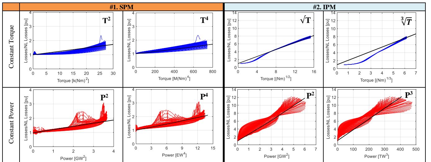
Fig. 9 Selection of the best exponent for modelling the ratio of iron loss to no-load loss versus load torque and power.
