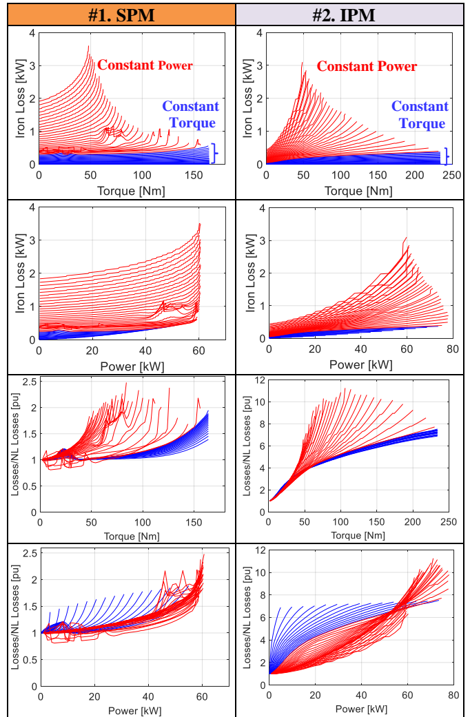
Fig. 8 Iron loss variation in the constant torque and constant power region versus torque and power, and effect of normalising the losses by the NL losses as a function of torque and power.
