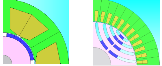
Fig. 2 Cross-sections of the two 50 kW machines (left SPM, right IPM).
