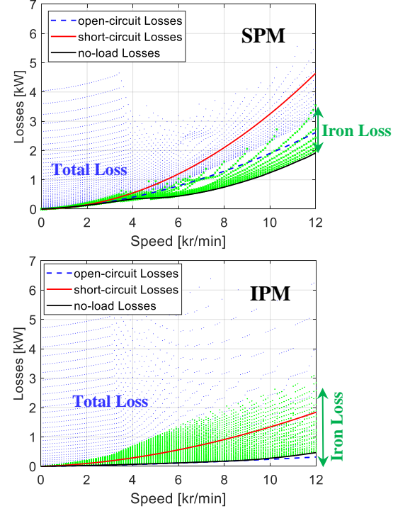
Fig. 5 Scatter plot of iron loss and total loss versus speed overlaid by the SC, OC, and NL losses versus speed curves (top SPM, bottom IPM).
