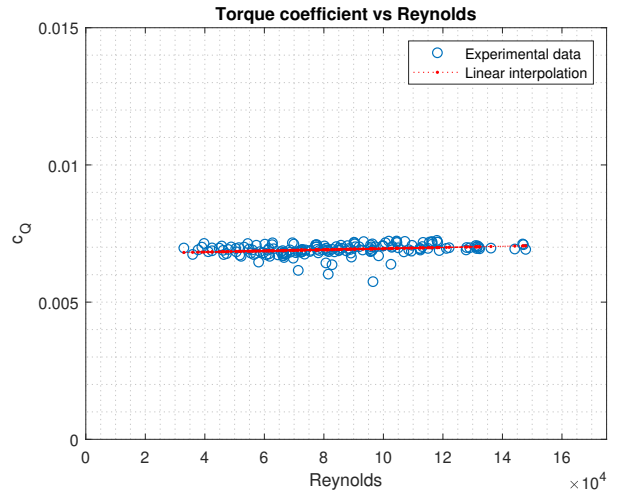
Fig. 10: Propeller torque coefficient and Reynolds number for all the temperature and pressure.
