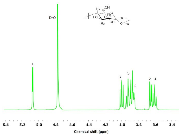
Figure S2: ^1\text{H-NMR} spectrum of \alpha -cyclodextrin.
