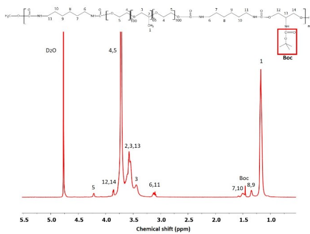
Figure S3: ^1\text{H-NMR} spectrum of as-synthesized NHP407.
