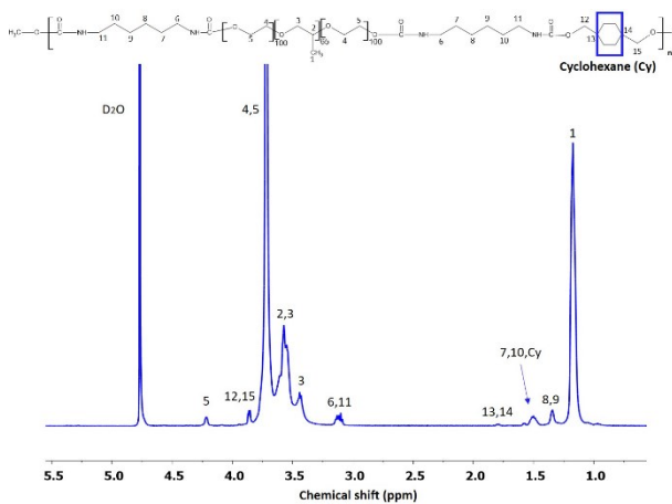
Figure S4: ^1\text{H-NMR} spectrum of as-synthesized CHP407.
