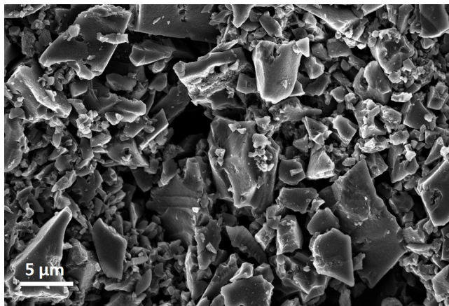
Figure 2: FESEM image of the activated carbon-based electrode.
