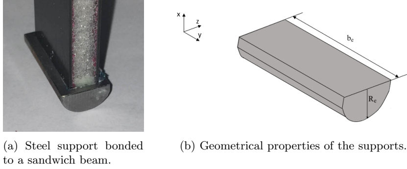
Fig. 2: Supports for simply-supported boundary conditions.
