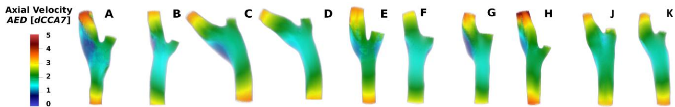
Fig. 7. “All-to-all” V_{ax} CNs. Volumetric maps of AED , i.e., the Euclidean length of persistence of correlated V_{ax} structures in the CB. AED is measured in terms of CCA7 diameters ( d_{CCA7} ), in order to account for CCA geometry inter-variability. Low AED values (below 1 d_{CCA7} ) at the carotid bulb reflect the impact of the bifurcation expansion in reducing the sphere of influence of axial flow in that region.
