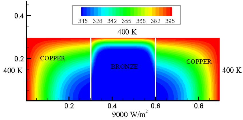
Figure 7. Temperature for copper-bronze blocks at t = 80 s
