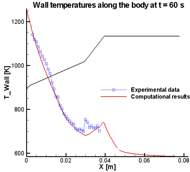
Figure 22. Computed and measured wall temperatures along the body at 60 \text{ s}
