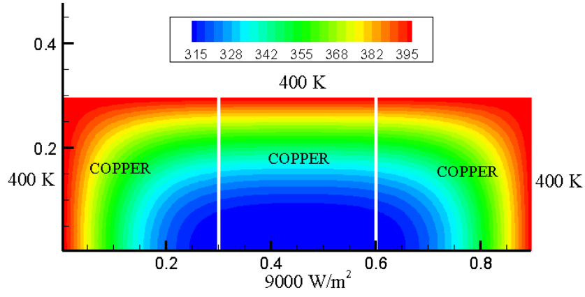
Figure 5. Temperature for three copper blocks at t = 80 s
