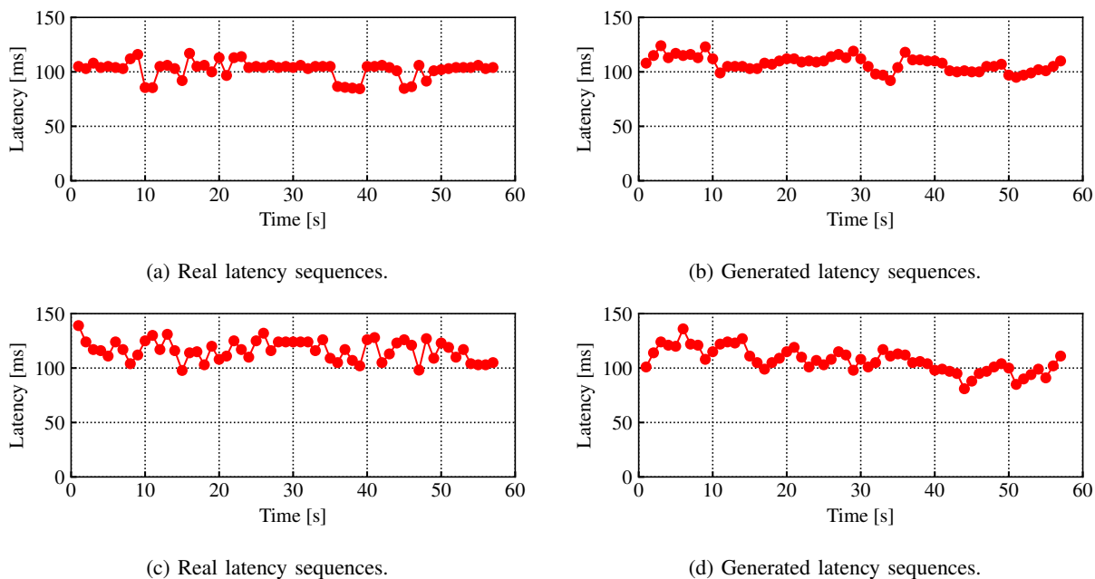
Fig. 3: Examples of real (left) and generated (right) latency sequences for the TIM, ordinary 3G profile.
