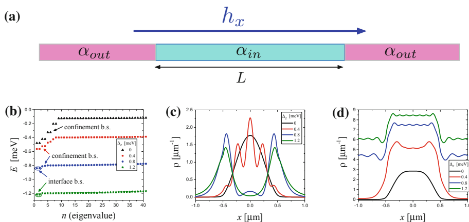
Fig. 5 Panel a : A 1\mu\text{m} -long portion of a InSb nanowire (effective mass m^* = 0.015m_e ) takes a RSOC value \alpha_{in} different from the value \alpha_{out} characterizing the rest of the nanowire, e.g. due to the presence of a metallic gate covering it. The RSOC \alpha_{in} corresponds to a bulk spin-orbit energy E_{SO,in} = 0.5\text{ meV} for the central region, while \alpha_{out} = -\alpha_{in}/2 , and E_{SO,out} = 0.125\text{ meV} . The smoothening length of the RSOC profile (13) is \lambda_s = 50\text{ nm} . The inhomogeneous nanowire is exposed to an external magnetic field along the nanowire axis. Panel b : The spectrum of the inhomogeneous nanowire is plotted for four different values of the applied magnetic field: for vanishing or weak magnetic field (black triangles and red squares) only confinement bound states are present. For \Delta_Z > \Delta_Z^* \simeq 0.5\text{ meV} , two additional interface bound states appear below the confinement bound states (blue circles), while for \Delta_Z > 2E_{SO} = 1\text{ meV} (green stars) the confinement bound states have disappeared and only the interface bound states survive. Panel c : The density profile \rho_{lowest} of the lowest energy state, plotted for the same four values of applied magnetic field, shows a change in the nature of the electronic ground state from a confinement to interface bound states, determining a displacement of the electron charge from the center to the interfaces with the leads located at x = \pm 0.5\mu\text{m} . Panel d : the profile of the total density \rho , involving all occupied states up to a chemical potential \mu = -0.45\text{ meV} is shown for the four different values of applied magnetic field
