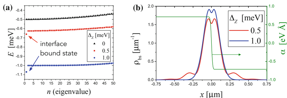
Fig. 4 Panel a : Energy spectrum of inhomogeneous RSOC profile (12) describing the interface sketched in Fig. 3, i.e. \alpha_L = \alpha and \alpha_R = -\alpha , with smoothening length \lambda_s = 50 nm, in a InSb nanowire ( m^* = 0.015m_e ). The spin-orbit energy characterizing both sides is E_{SO} = 0.5 meV and the three different curves refer to three different values of the magnetic gap energy \Delta_Z = |h_x| . While for vanishing magnetic field the spectrum has a purely continuum branch, for non-vanishing magnetic field a bound state appears below the continuum branch. Panel (b) : the density profile of the bound state is plotted for the two non-vanishing magnetic field values, showing that the bound state is located at the interface. The thin green curves describes the RSOC profile Eq. (12)
