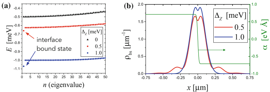
Fig. 4 Panel a : Energy spectrum of inhomogeneous RSOC profile (12) describing the interface sketched in Fig. 3, i.e. \alpha_L = \alpha and \alpha_R = -\alpha , with smoothing length \lambda_s = 50 nm, in a InSb nanowire ( m^* = 0.015m_e ). The spin-orbit energy characterizing both sides is E_{SO} = 0.5 meV and the three different curves refer to three different values of the magnetic gap energy \Delta_Z = |h_x| . While for vanishing magnetic field the spectrum has a purely continuum branch, for non-vanishing magnetic field a bound state appears below the continuum branch. Panel (b) : the density profile of the bound state is plotted for the two non-vanishing magnetic field values, showing that the bound state is located at the interface. The thin green curves describes the RSOC profile Eq. (12)
