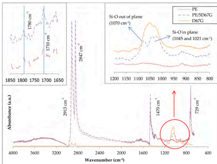
Figure 2. ATR-FTIR spectra of Dellite 67G, PE and PE/5D67G as-spun fibers in the range 600\text{--}4000\text{ cm}^{-1} . Detail of the regions 1650\text{--}1850\text{ cm}^{-1} and 800\text{--}1200\text{ cm}^{-1} are also reported.
