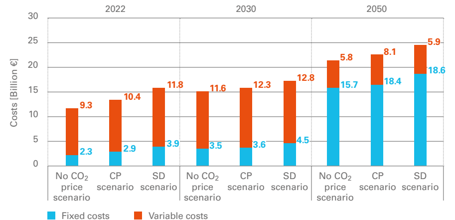
Figure 18 Generation system costs in different scenarios. Variable costs for all units. Fixed costs include fixed O&M for all units, and capital costs for new units.
