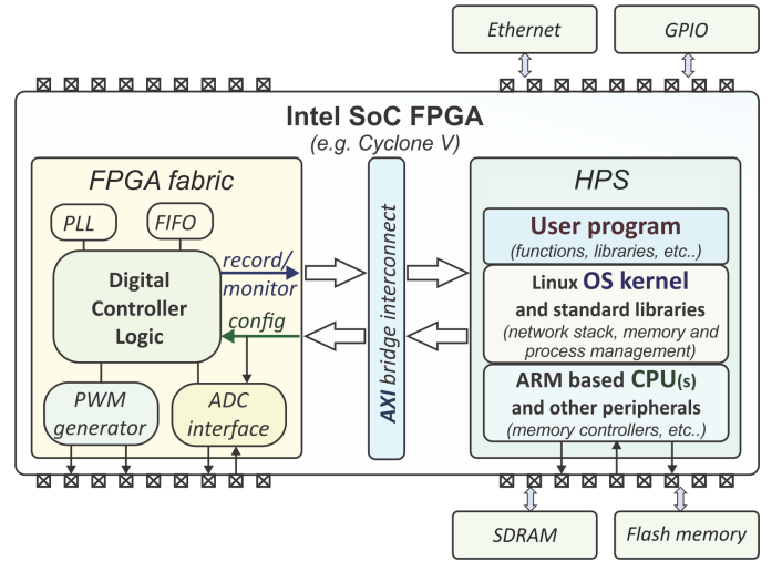
Figure 3. Basic internal modules of Intel SoC package (e.g. Cyclone V) used to build a digital controller. FPGA and HPS fabric communicate through built-in AXI (Advanced eXtensible Interface) bridge. FPGA part implements digital controller, while HPS performs configuration and monitoring/recording (see also Fig.2). ADC interface logic written in HDL interacts with external ADC chip
