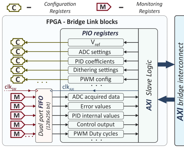
Figure 5. Section of AXI interface blocks inside FPGA. Set of Programmable Input-Output (PIO) registers are used to connect FPGA blocks with built-in AXI bridge interconnect. PIO registers are seen as slave peripherals from HPS side. "Monitoring" data are fed to the HPS through Dual-port FIFO for synchronization.
