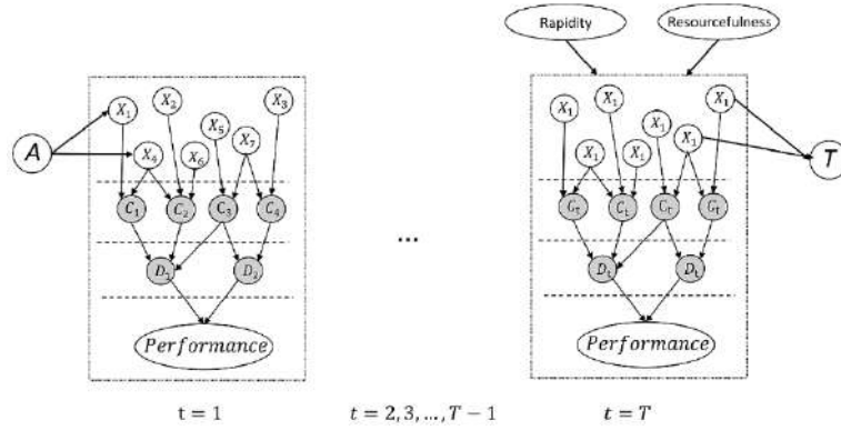
Figure 21 Bayesian network with additional variables in the first and last slices
