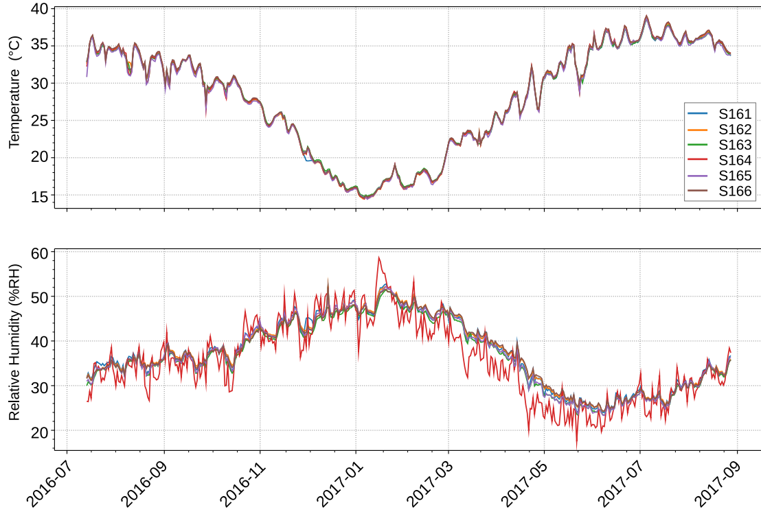
Fig. 4. T and RH measurements collected for one year during the Sohag Museum monitoring campaign from the smart sensors inside (S161, S162, S163, S165, S166) and outside (S164) the showcases.
