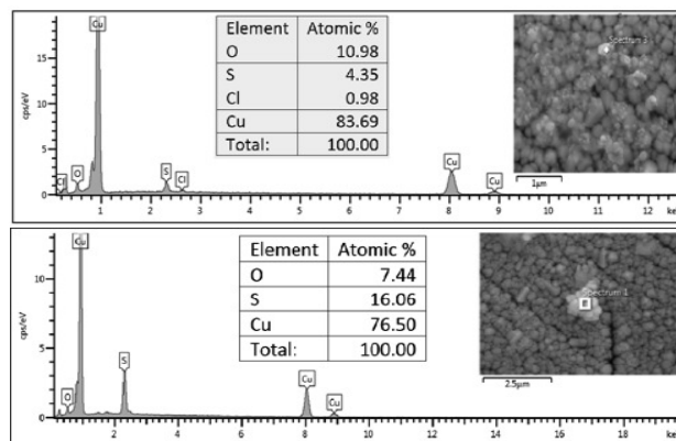
Fig. 8. Chemical composition of the corrosion products detected by the quantitative SSD probe on the Cu reference specimens positioned near sensor S162 after 2 months (top) and 6 months (bottom) of exposure to the showcase atmosphere, respectively (as an example).
