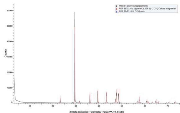
Fig. 5. XRD of limestone taken from Pidiego quarry.
