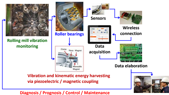
Fig. 7. Concept of smart bearing for large equipment monitoring with embedded sensors and autonomous energy supply.
