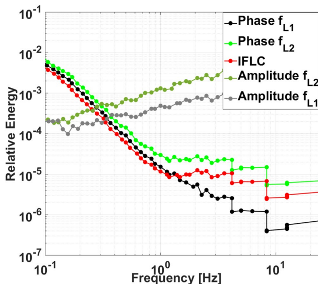
Fig. 5 Power spectral densities of phases, amplitudes of GPS L1 and L2 and IFLC for Case 2. No cutoff frequency is identified
