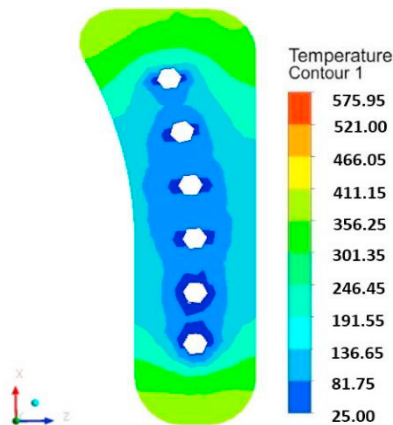
Fig. 14. Thermal field in the core of the insert [°C].
