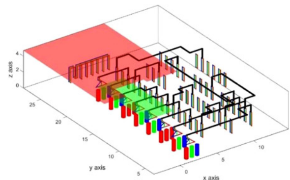
Fig. 11 3D Model of the substation in presence of the two shields
