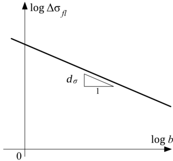
Figure 3: Specimen-size effects on fatigue limit in a bi-logarithmic diagram
