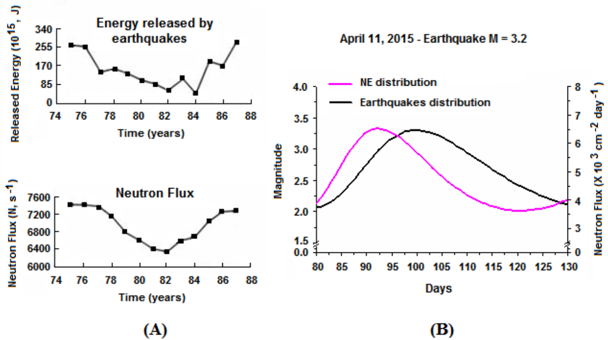
Figure 3. (A) Seismic activity and neutron flux measurements in the period 1975–1987 (Kola Peninsula, Russia [33]); (B) Typical time correlation between fitting distributions of neutron flux measurements at the Murisengo gypsum mine, and a local seismic swarm (magnitude 3.2 main shock) [36].
