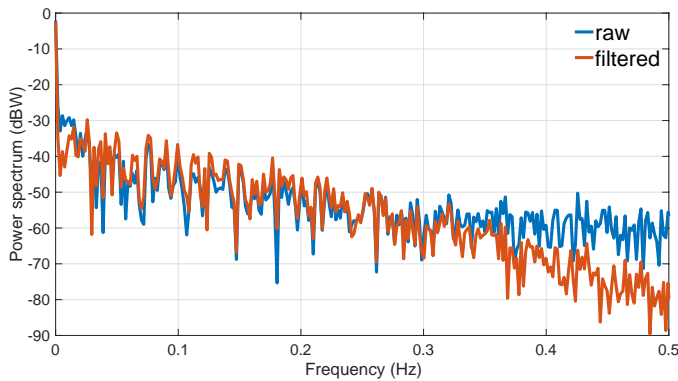
Fig. 6. Power frequency spectrum of one sensor output before (“raw”) and after digital filtering (“filtered”). The median filter attenuates frequencies below 0.02 Hz and the low-pass filter attenuates frequencies above 0.3 Hz.
