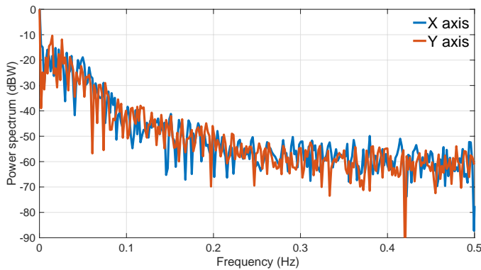
Fig. 7. Power frequency spectrum of the reference localization system output coordinates, X and Y. Below 0.3 Hz the signal rises above the noise floor and increases especially at lower frequencies, corresponding to slow movements.
