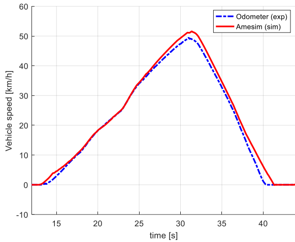
Figure 12. Vehicle speed.
