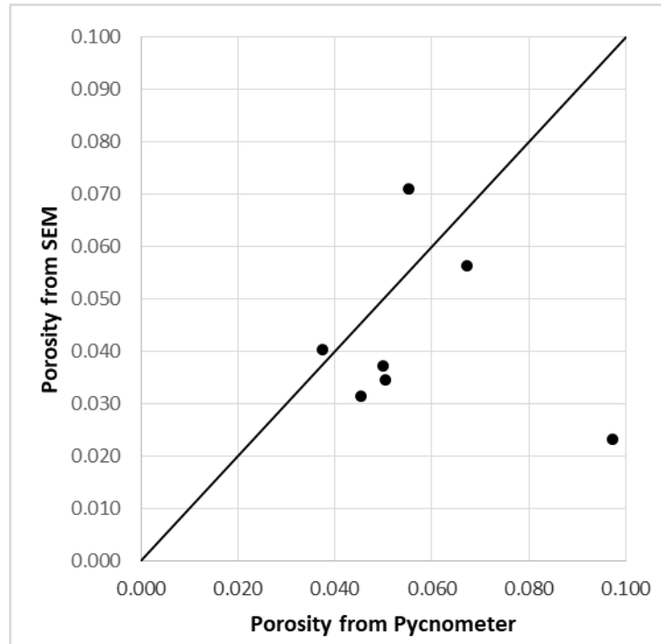
Figure 5 Comparison among porosity results measured with image analysis method and with helium pycnometer
